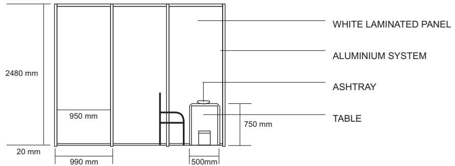
SIDE SECTIONAL ELEVATION
