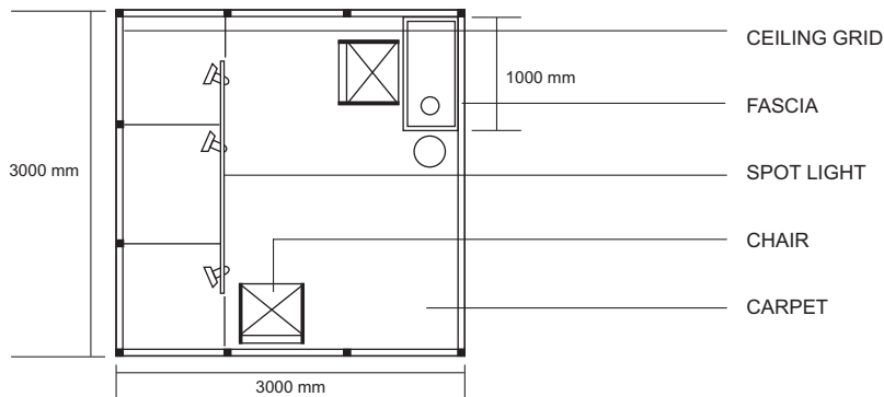
FLOOR PLAN
